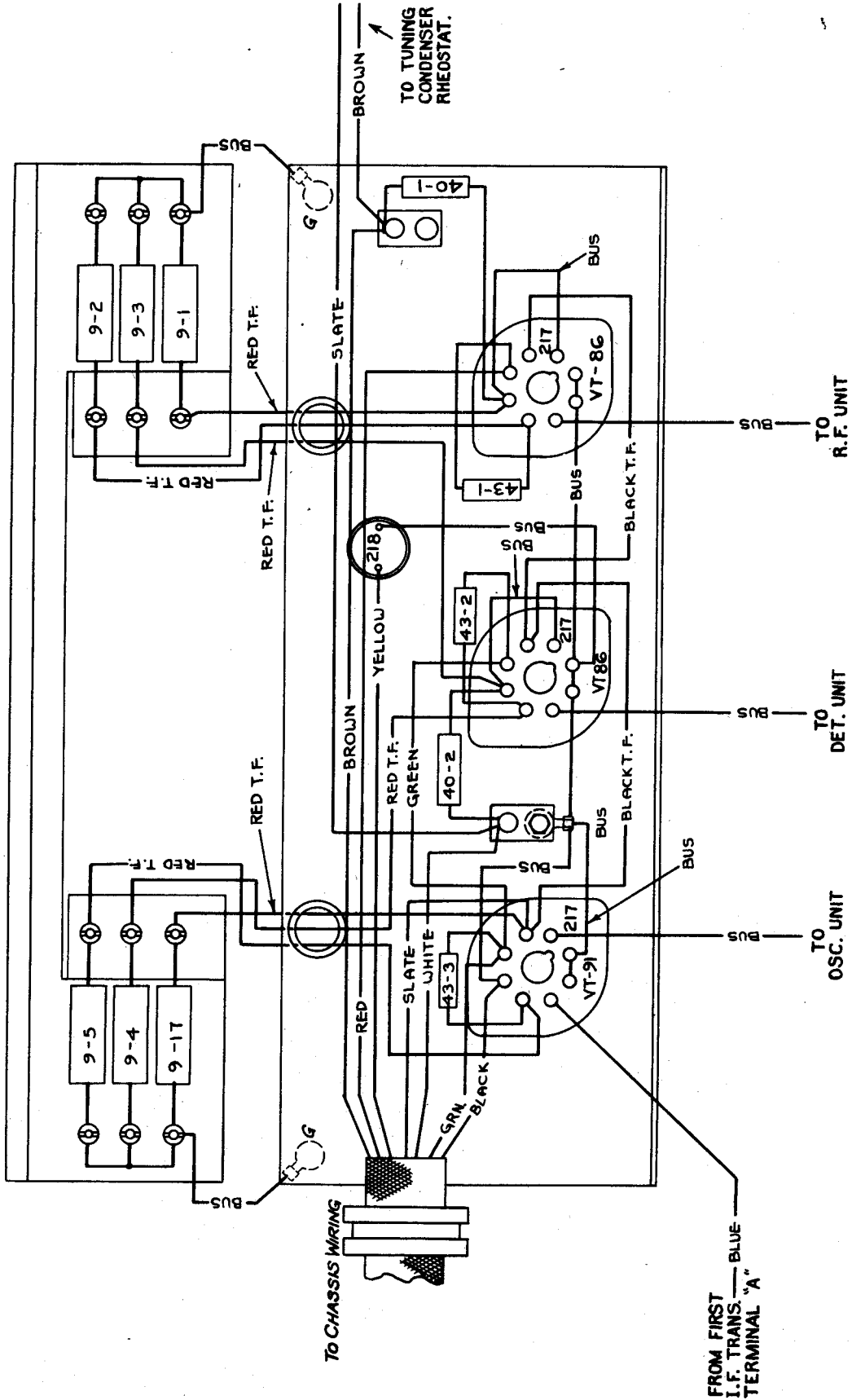
Figure 32 — Radio Receiver BC-224-1*, Wiring Diagram, Tube Shelf
